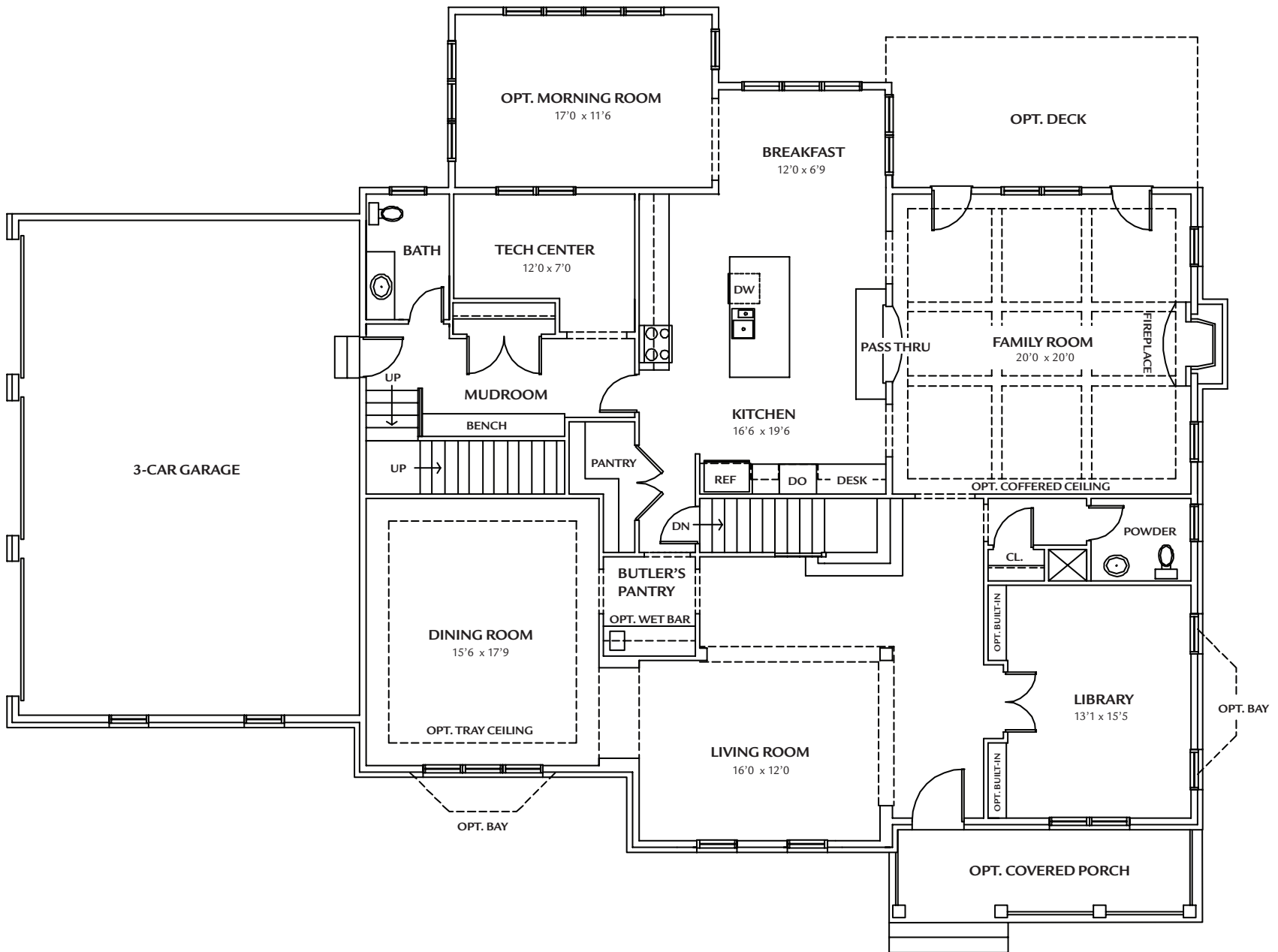
First Floor
